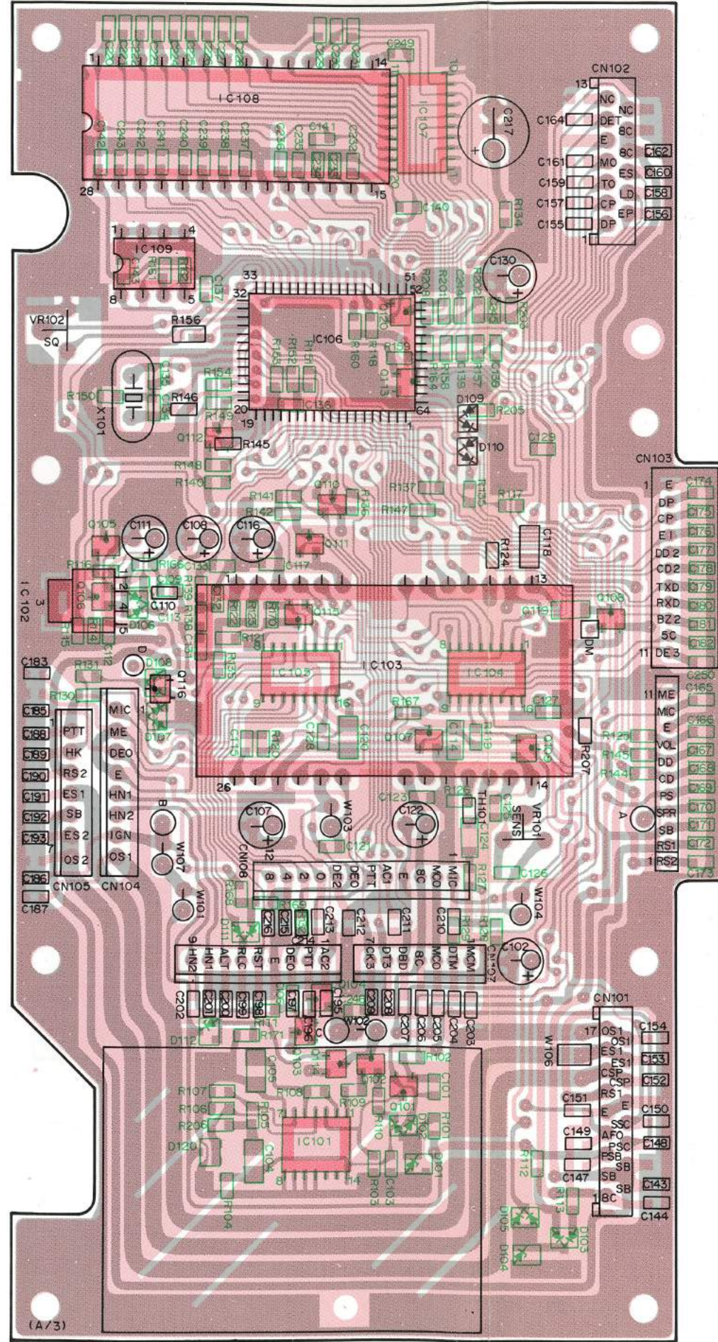
TX-RX UNIT (X57-3750-10) Foil side view
