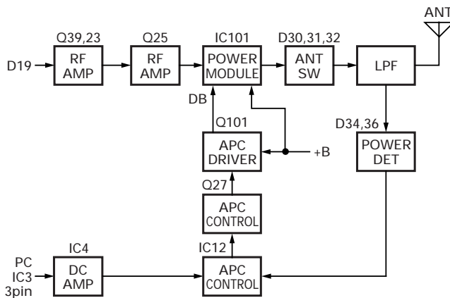
Fig. 9 APC circuit
