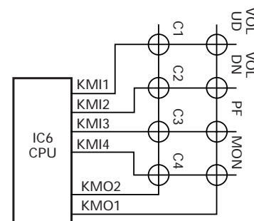
Fig. 13 Key matrix circuit
