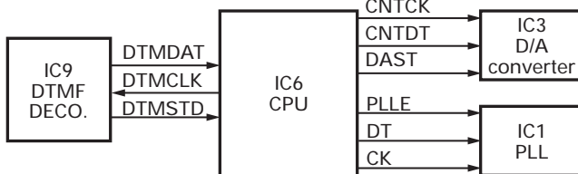
Fig. 10 Control circuit
